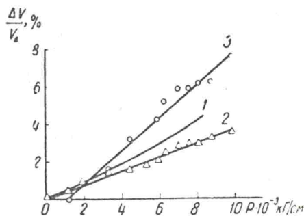
FIG. 4. Relative volume change of \gamma - and \alpha -phases of cerium vs. pressure: (1) for \gamma -phase (according to Bridgman); (2) \gamma -phase (according to us); (3) for \alpha -phase (according to us).
